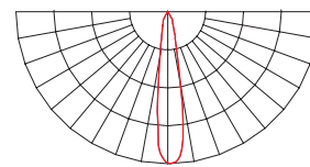
10° LOR 87%
