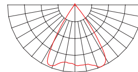
70° LOR 87%
