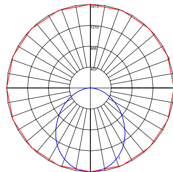
NRLED Diffuser
